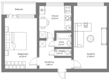
Buto planas 46.76 m 2
